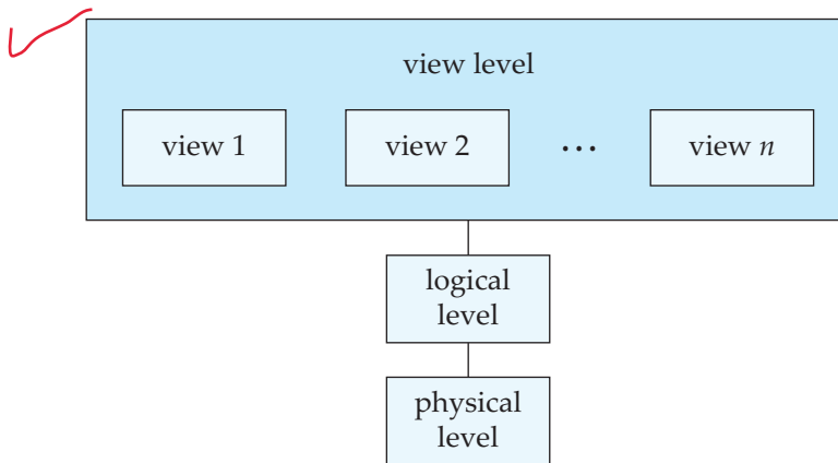
Figure 1.1 The three levels of data abstraction.
