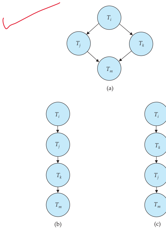
Figure 14.12 Illustration of topological sorting.
