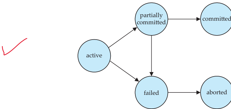
Figure 14.1 State diagram of a transaction.
