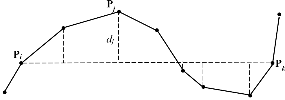
Fig. 6.18 Polygon approximation by merging
