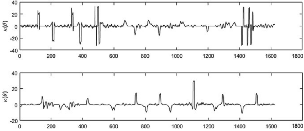
Fig. 6.10 Curvature signatures. Top: curvature signature of a tree shape from Fig. 6.7 without smoothing; bottom: curvature signature of the same tree shape with a Gaussian smoothing
