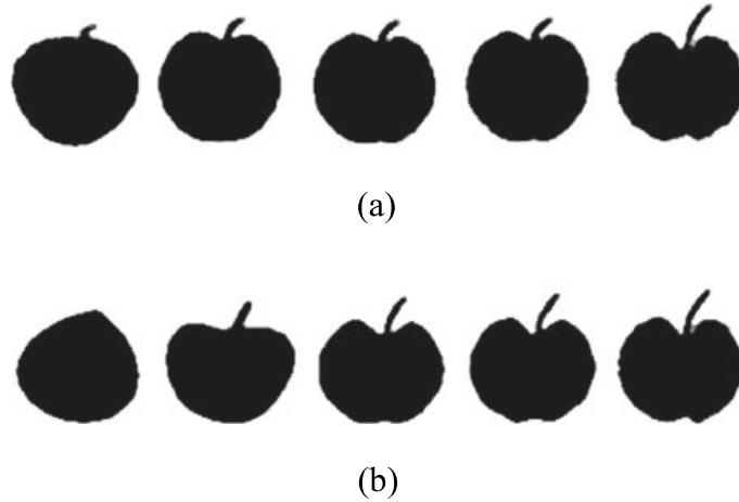
Fig. 6.16 Reconstructed shapes of an apple shape using Fourier coefficients from a r(t) and b z(t) . In both (a) and (b), from left to right, the shapes are reconstructed using 5, 10, 20, 30 and all the Fourier coefficients, respectively
