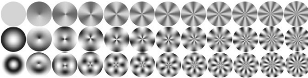
Fig. 6.24 Real parts of the ART basis functions
