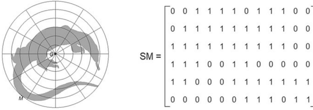
Fig. 6.28 Computation of a polar raster shape matrix. Left: Polar raster sampling of a shape; Right: Its polar shape matrix
