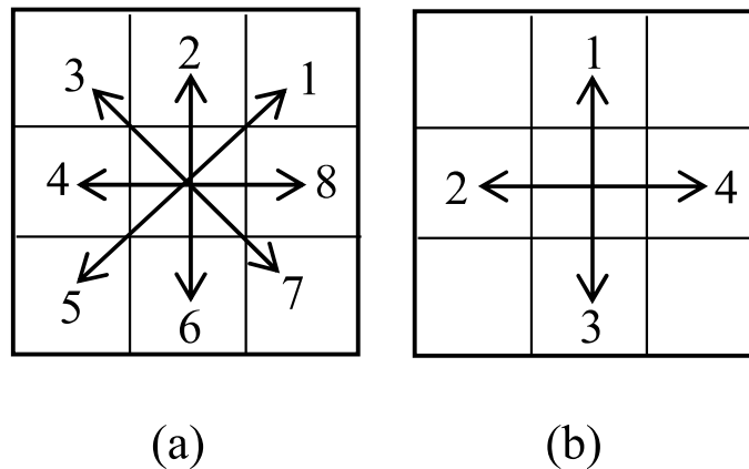
Fig. 6.20 Computation of chain code. a Chain code in 8-connectivity; b chain code in 4-connectivity
