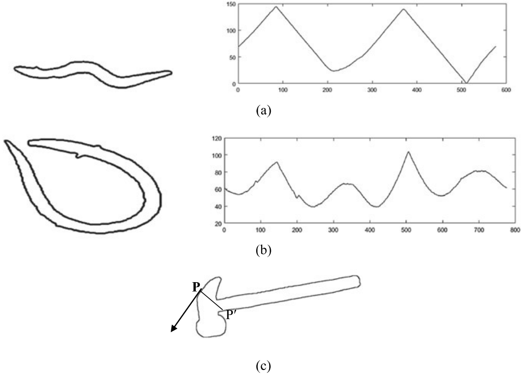
Fig. 6.8 Computation of chord length signature. a A sea snake shape on the left and its r(t) function on the right; b another sea snake shape on the left and its r(t) function on the right; c illustration of computing r^*(t) at point P of a hammer shape
