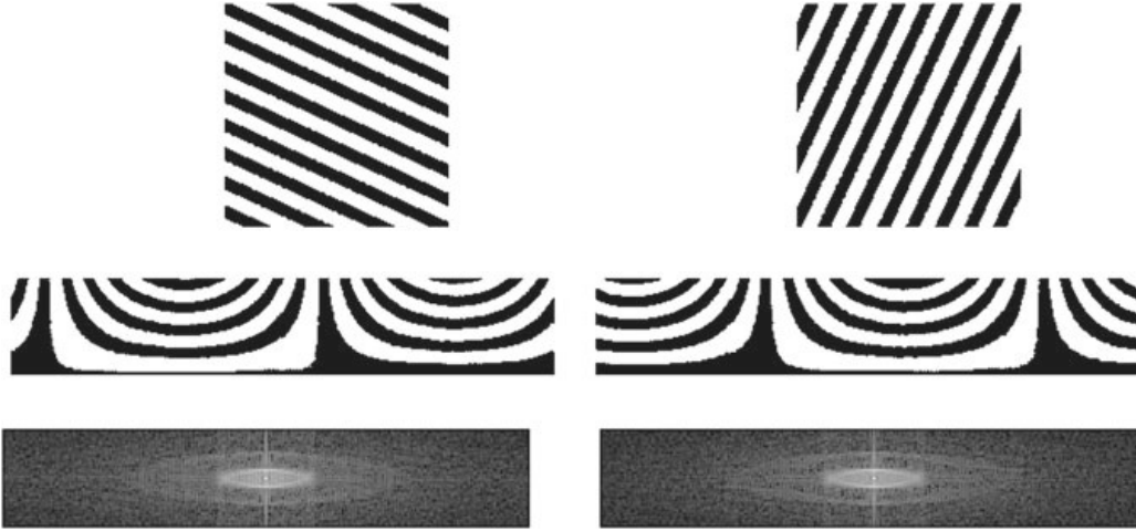
Fig. 6.26 Rotation-invariant GFD. Top row: Two shape images with different orientations; Middle row: The polar raster-sampled images of the two corresponding shapes at the top row; Bottom row: The Fourier spectra images of the two corresponding images at the middle row
