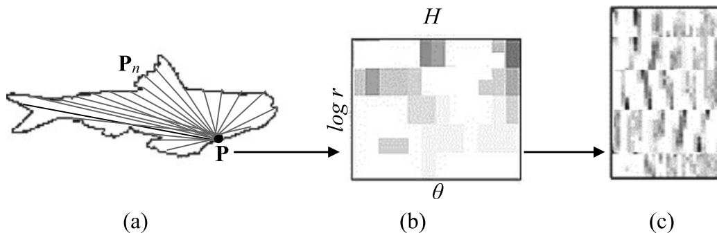
Fig. 6.12 Computation of shape context. a A point \mathbf{P} on a shape boundary and all the vectors started from \mathbf{P} ; b the log-polar histogram H of the vectors from \mathbf{P} , the histogram H is the context of point \mathbf{P} ; c the shape context map of shape of (a), each row of the context map is the flattened histogram of a point context, the number of rows is the number of sampled points
