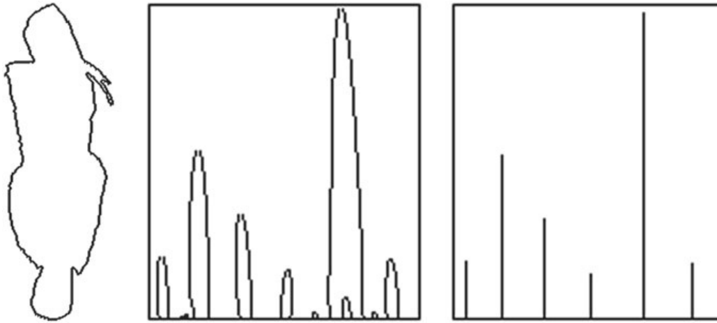
Fig. 6.14 Computation of curvature scale space. A fish shape ( left ), its CSS contour map ( center ) and CSS peaks ( right )
