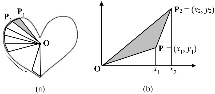
Fig. 6.11 Computation of area signature. a Triangulation of a heart shape; b illustration on the calculation of the area of the shaded triangle
