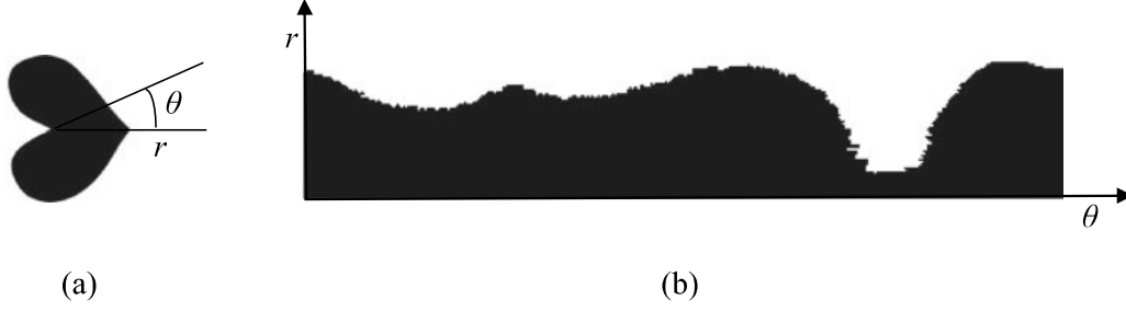
Fig. 6.25 Polar raster transform. a An original shape image in polar space; b polar raster-sampled image (a) plotted into Cartesian space
