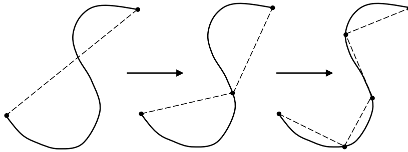
Fig. 6.19 Polygon approximation by splitting
