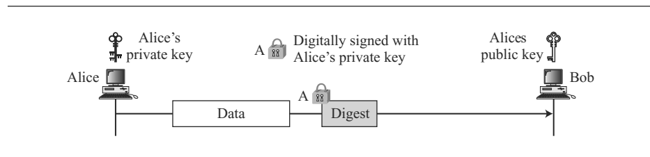
Figure 16.3 An authenticated message
