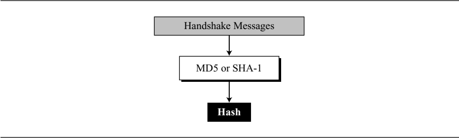
Figure 17.44 Hash for CertificateVerify message in TLS
