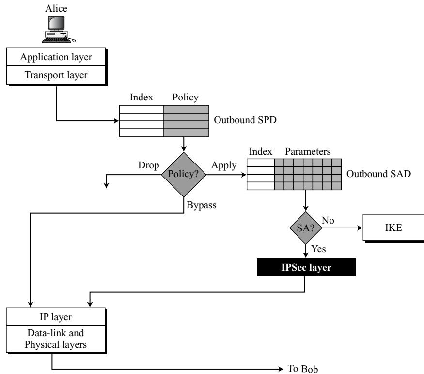
Figure 18.13 Outbound processing
