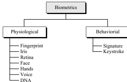
Figure 14.17 Biometrics
