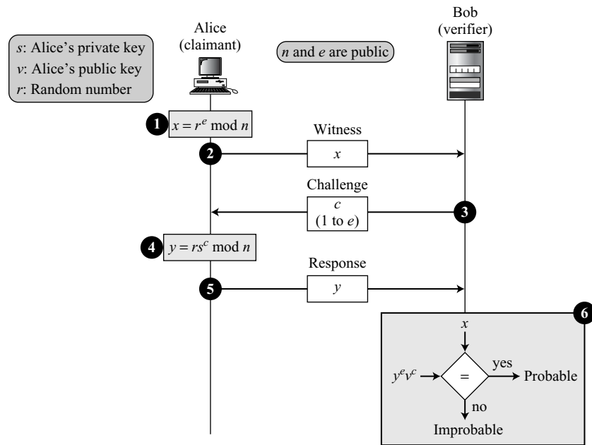
Figure 14.16 Guillou-Quisquater protocol
