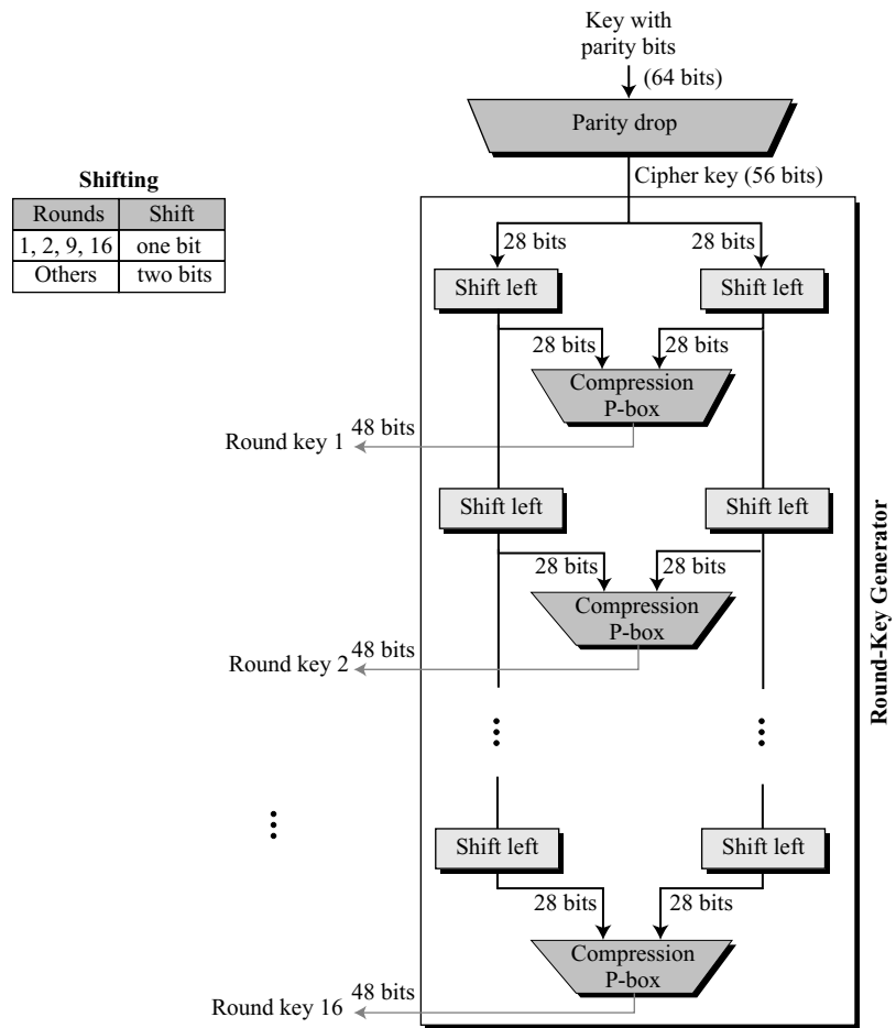
Figure 6.10 Key generation
