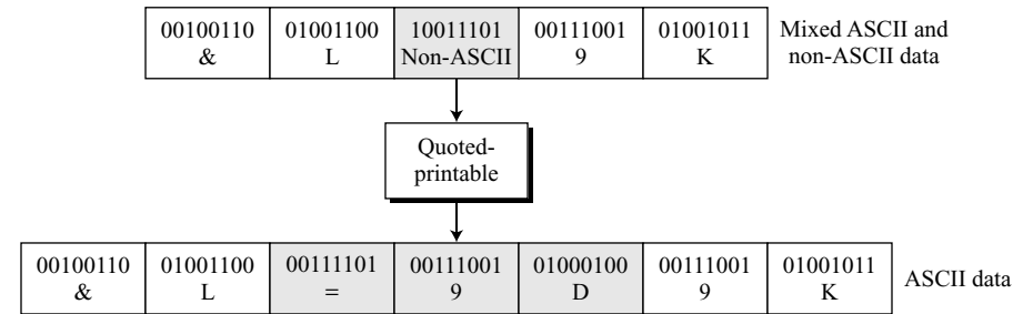
Figure 16.26 Quoted-printable
