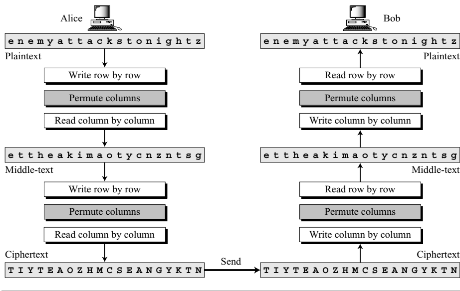
Figure 3.25 Double transposition cipher
