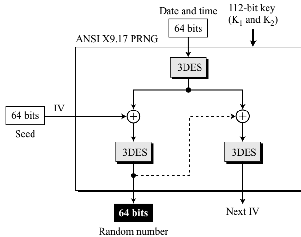
Figure K.4 ANSI X9.17 pseudorandom number generator
