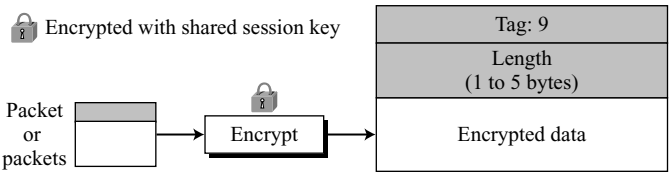
Figure 16.15 Encrypted data packet
