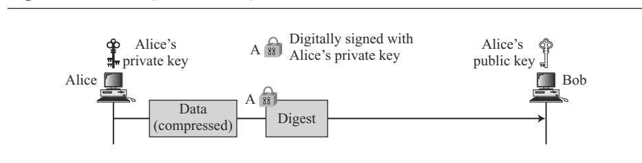
Figure 16.4 A compressed message
