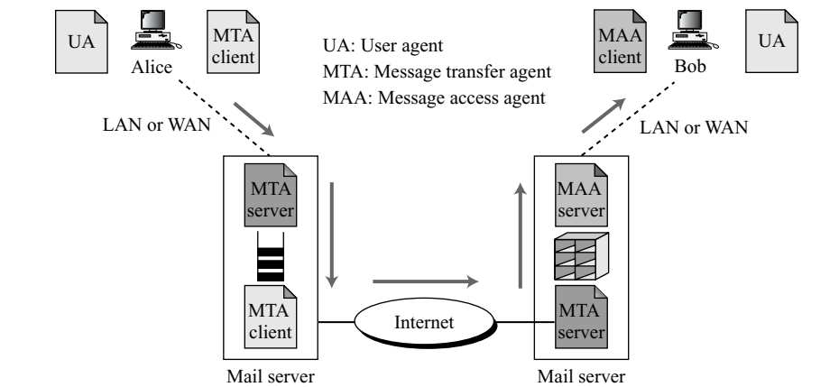
Figure 16.1 E-mail architecture
